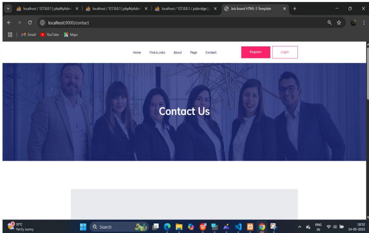
Fig 7.6: Contact Us
