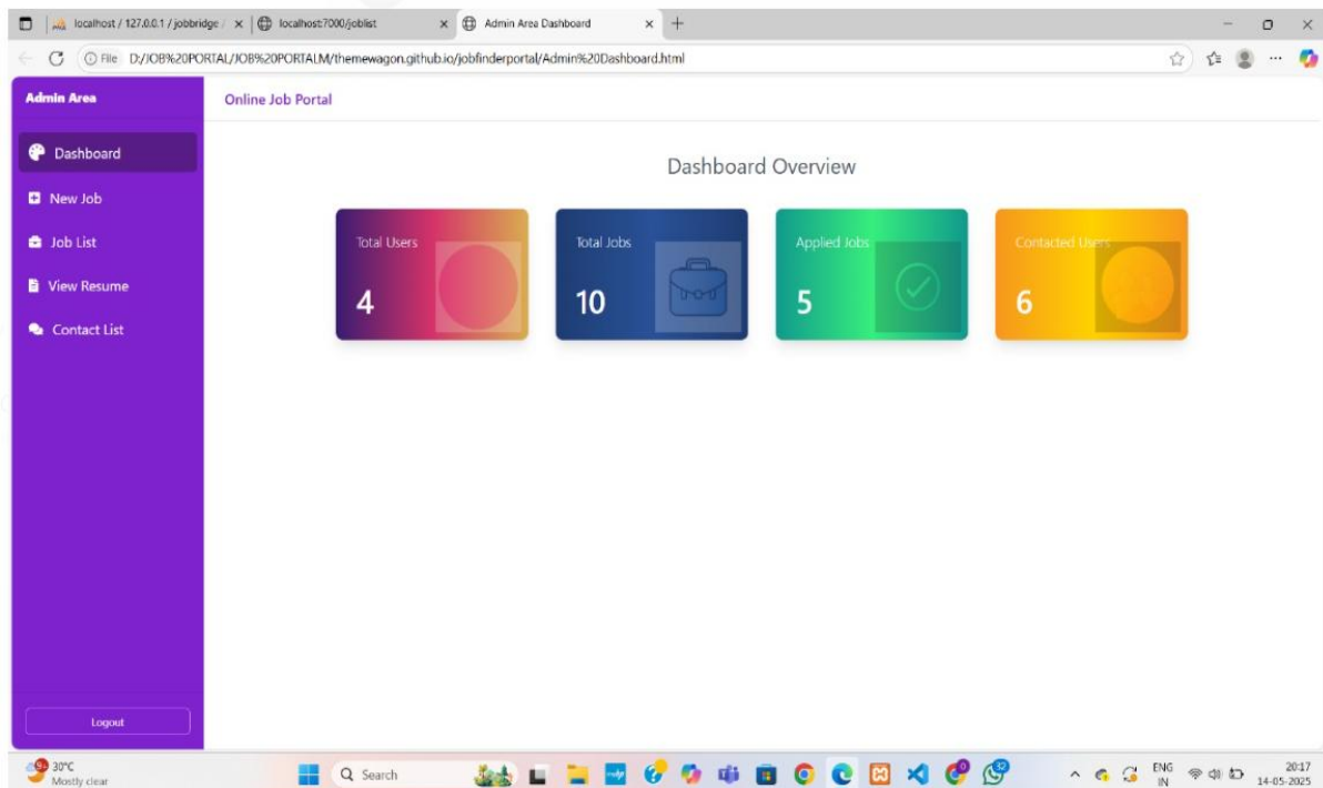
Fig 7.7: Dashboard Overview
