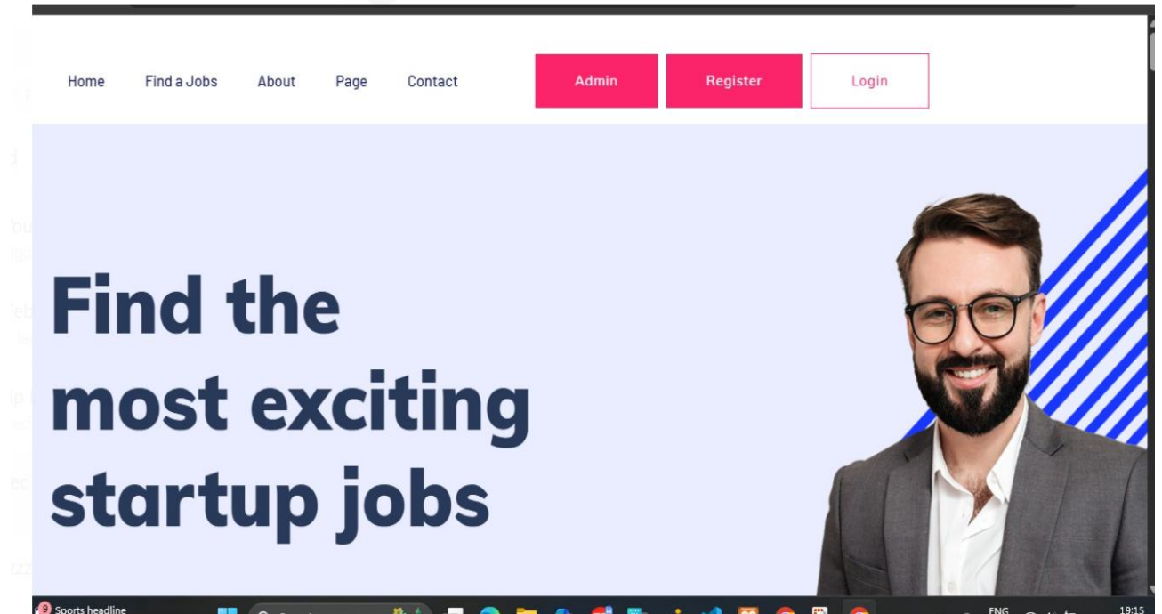
Fig 7.1: Home Page
